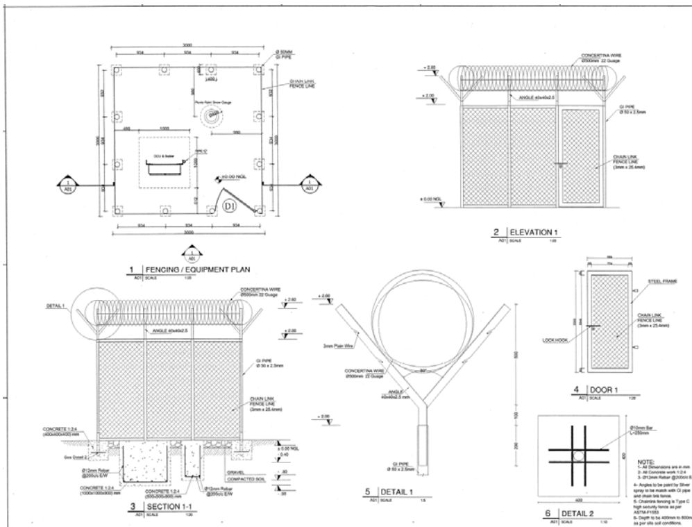
Figure 4 Typical Drawing for Fencing Stations
