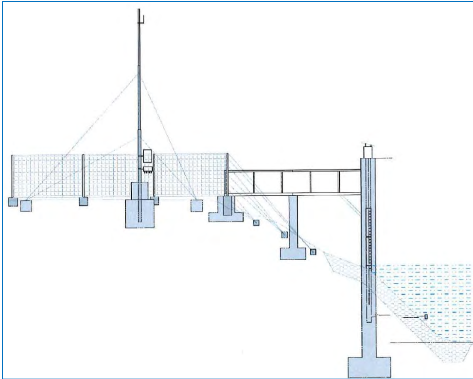
Figure 3 Sketch of hydrometric or gauge station
