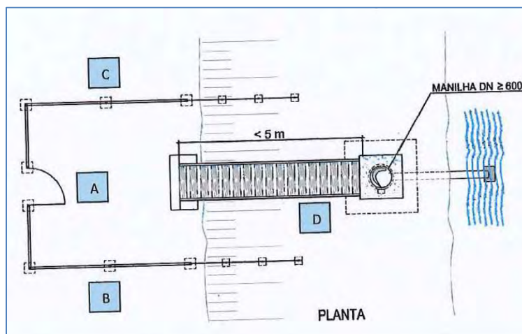
Figure 1 Typical Drawing for Fencing and Gauging Stations
